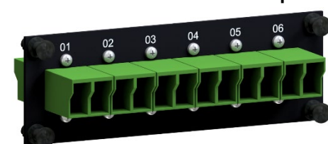
1 HE 1/4 TFP 6 E-2000®-Compact
